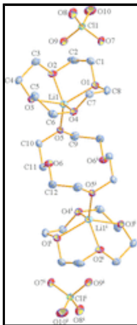
Fig. 1. Molecular structure of (I). The thermal ellipsoids are shown at 50% probability level. All hydrogen atoms were omitted for clarity. Symmetry transformations used to generate equivalent atoms: i -x, -y, -z+2 .
